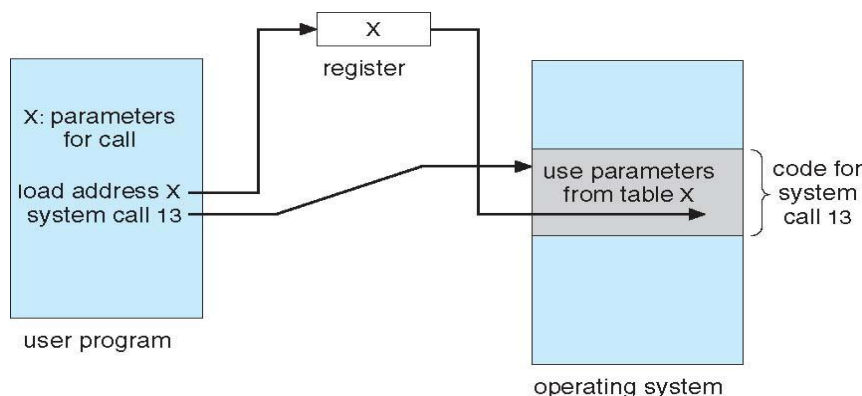
Figure: Passing of parameters as a table.
