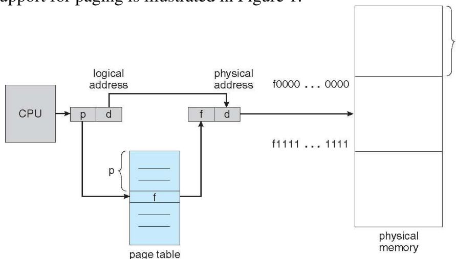
Figure 1: Paging hardware
