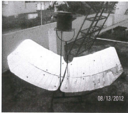
Butterfly design Solar Cooker
