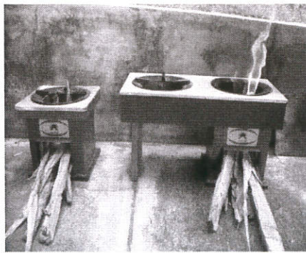
Single and Double high efficiency Chula
