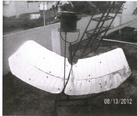
Butterfly solar cooker
